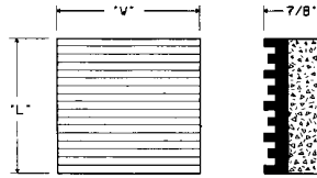
SERIES "NNP" RIBBED NEOPRENE ISOLATION PAD
