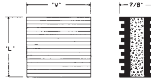
SERIES "NNP" RIBBED NEOPRENE ISOLATION PAD
